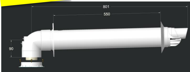
Kit Standard 60/100-60/100
