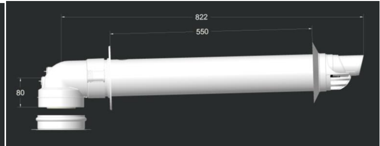
Kit Standard 80/125-60/100
